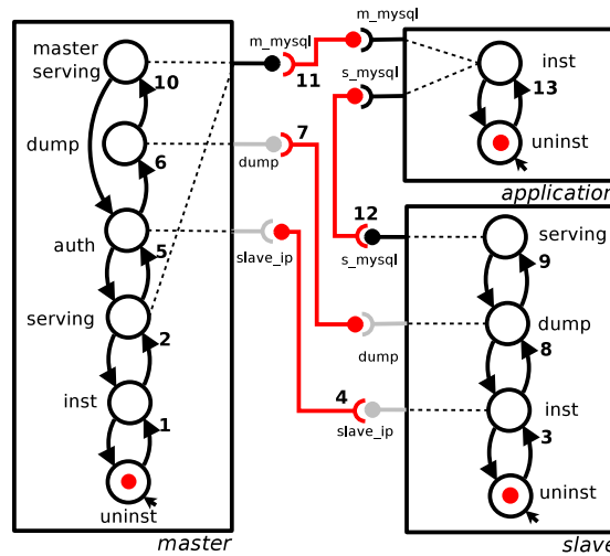
Figure 3: Sample deployment plan for the running example.
