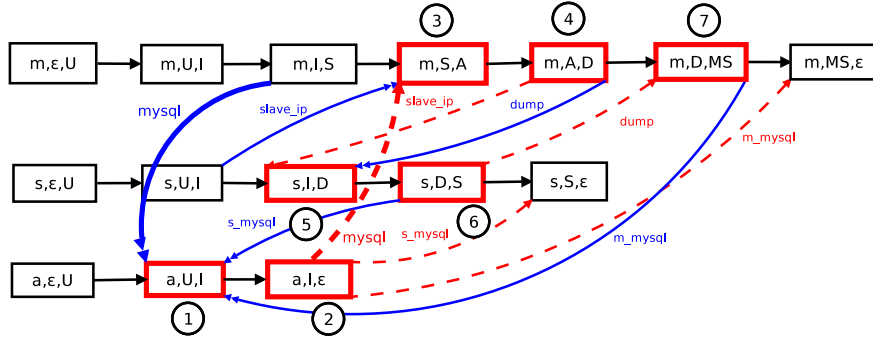
Figure 8: Cyclic abstract plan for the modified running example.
