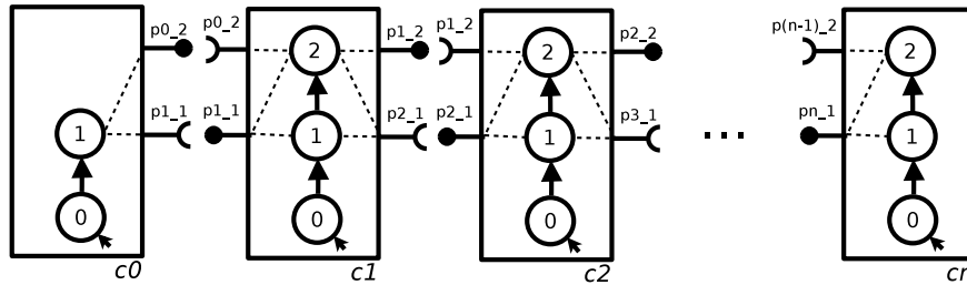
Figure 10: Component types for the validation with artificial instances.
