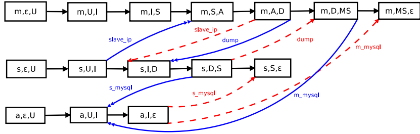
Figure 6: Abstract plan for the running example.
