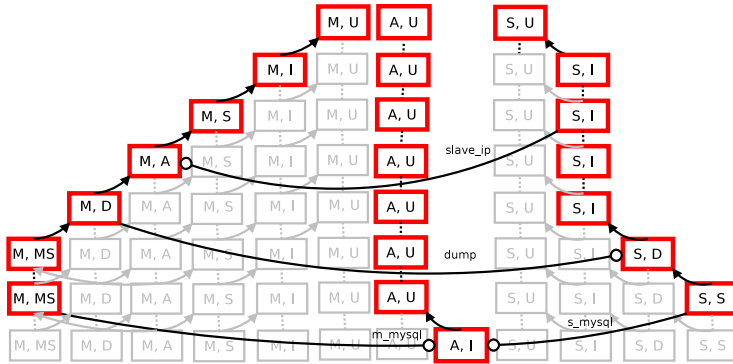
Figure 4: Reachability graph and component selection for the running example.
