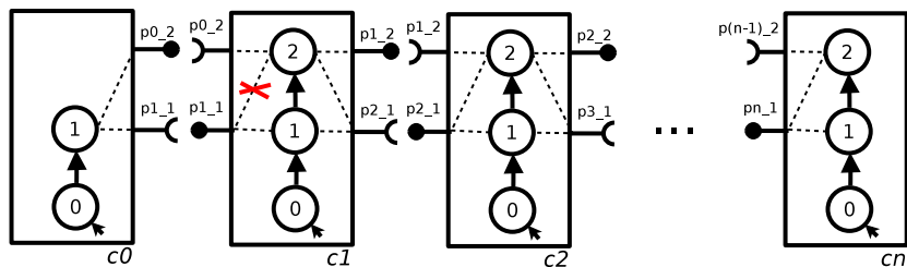
Figure 11: Modified version requiring duplication.
