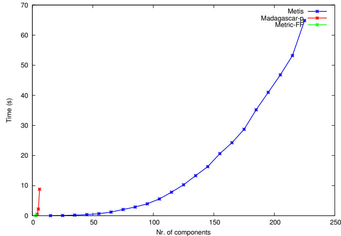
Figure 12: METIS vs. general purpose planners for scenarios without duplication.
