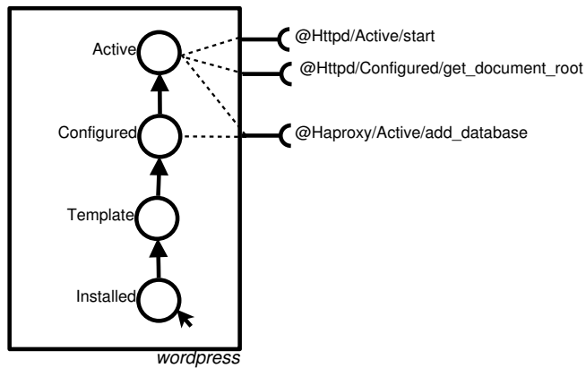
Figure 14: Aeolus WordPress component generated automatically by Blender.
