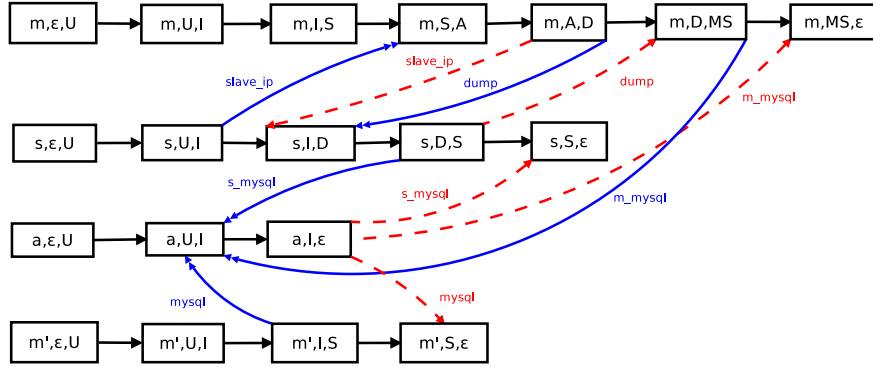
Figure 9: Effect of the duplication of node \langle m, S, A \rangle in Figure 8.
