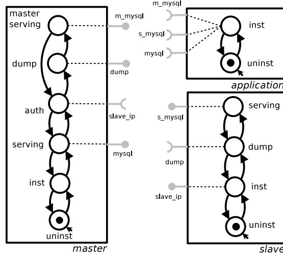
Figure 7: Component types for the new scenario requiring duplication.
