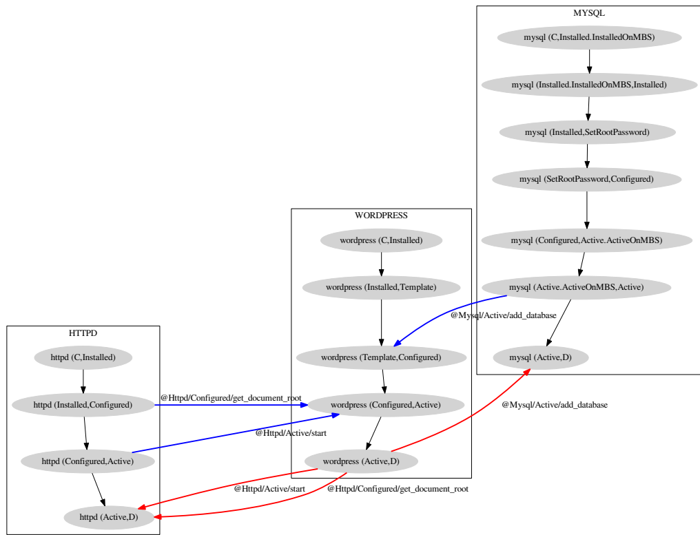
Figure 15: Abstract plan generated by METIS.
