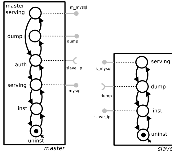
Figure 1: MySQL master-slave components according to the Aeolus model.
