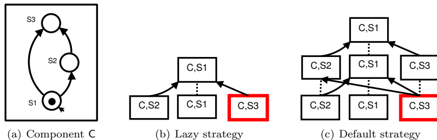
Figure 5: Difference between lazy and default strategies.
