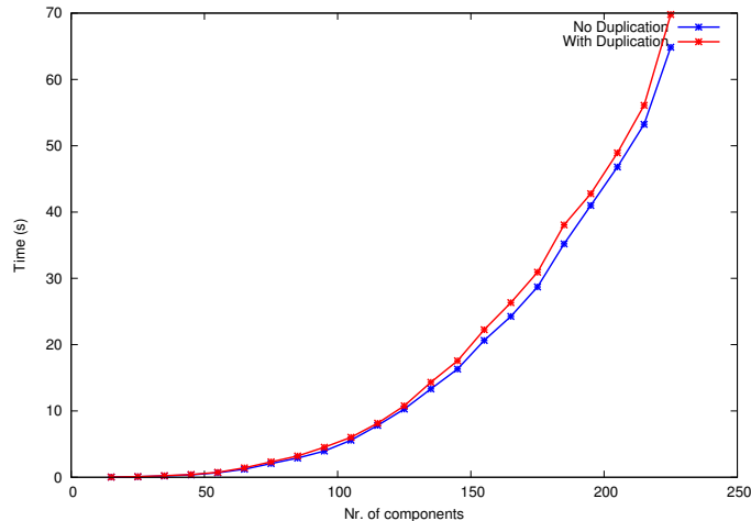
Figure 13: Performance of METIS for scenarios with and without duplication.
