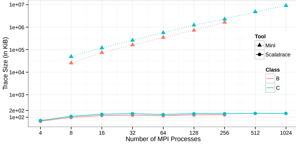
Figure 4: Evolution of the trace size in the MinI and ScalaTrace formats for different instances of the LU benchmark.
