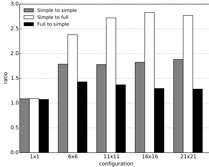
Figure 13: With-adaptiveness-over-without-adaptiveness ratio.
