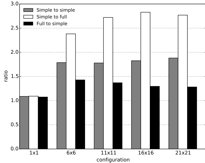
Figure 13: With-adaptiveness-over-without-adaptiveness ratio.
