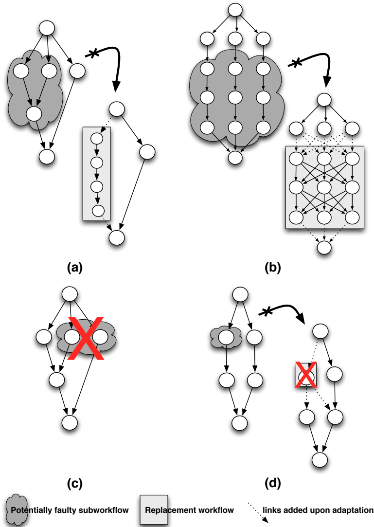
Figure 9: Valid and invalid cases of adaptations.
