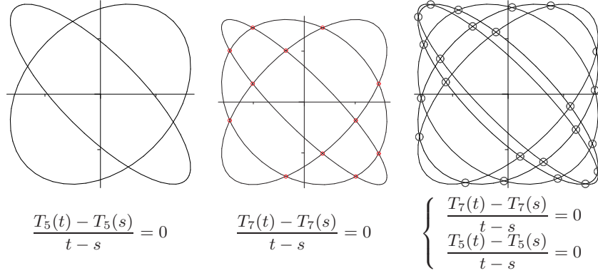
Figure 5: Double points in the parameter space
