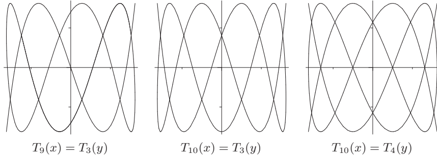
Figure 4: Implicit Chebyshev curves
