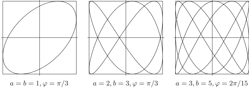
Figure 3: Lissajous curves x = 2 \cos at, y = 2 \cos(bt + \varphi)
