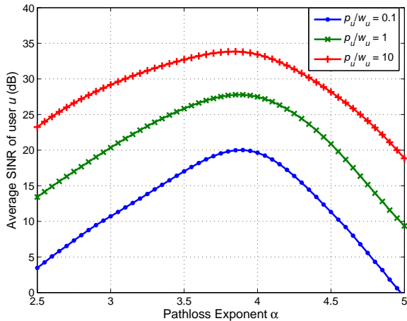
Fig. 8. Average SINR as a function of the path loss exponent for a user u with allocated resources (w_u, p_u) (ratio p_u/w_u in \text{W/MHz} ).
