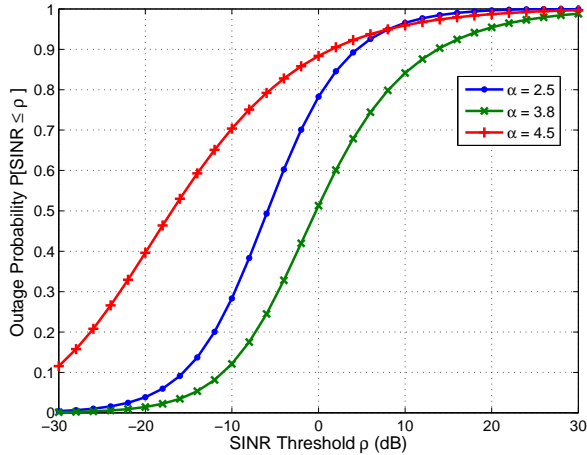
Fig. 7. SINR cdf as a function of the path loss exponent for a user u with p_u/w_u = 2\text{W/MHz} .
