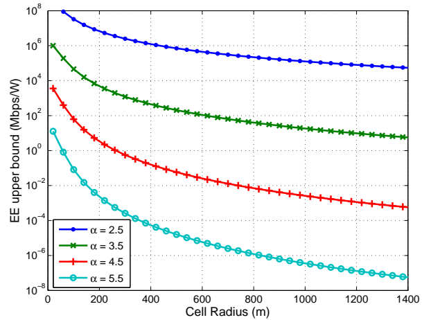
Fig. 6. EE upper bound EE^* from (17) in the low SNR regime as a function of the path loss exponent and the cell radius.
