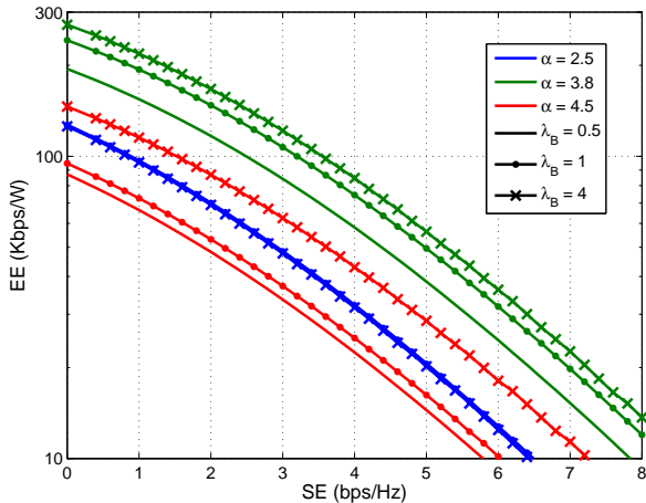
Fig. 9. Multi-cell SE-EE trade-off from (P_4) as a function of the path loss exponent and the BS density ( \lambda_B in points/ \text{km}^2 ).
