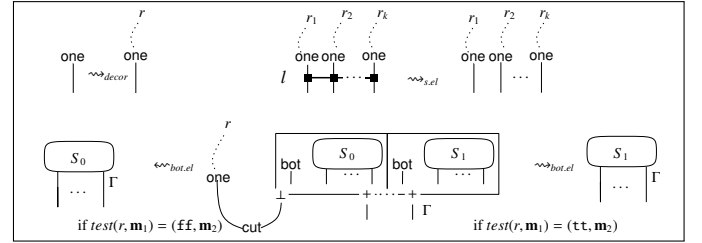
Fig. 10. Program Net Rewriting.
