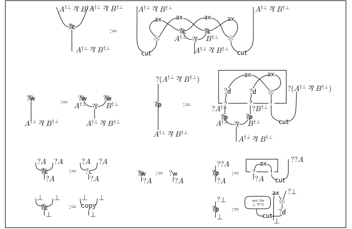
Fig. 16. Inductive Definition of Contraction, Weakening and Promotion Nodes.
