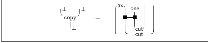
Fig. 13. Syntactic Sugar: Copying \perp .
