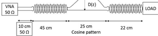
Fig. 3: Experimental setup. The cosine profile is inserted between two 110\ \Omega twisted pair segments.
