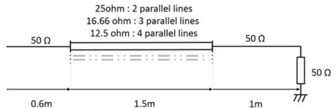
Fig. 11: Topology of the composite lines used. Equivalent cables of characteristic impedance smaller than 50 \Omega are realized by putting multiple 50 \Omega coaxial cables in parallel.
