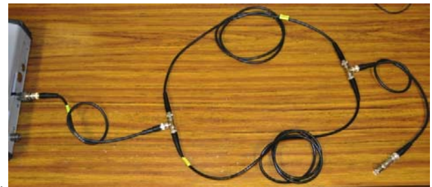
Fig. 10: Composite line including two RG-58 50 \Omega coaxial cables in parallel.
