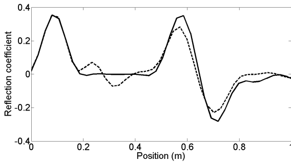
Fig. 4: Simulated (-) and experimental (- -) impulse responses of the cable illustrated in Fig. 3.
