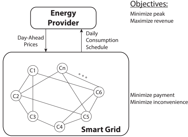
Figure 1: Bilevel Structure
