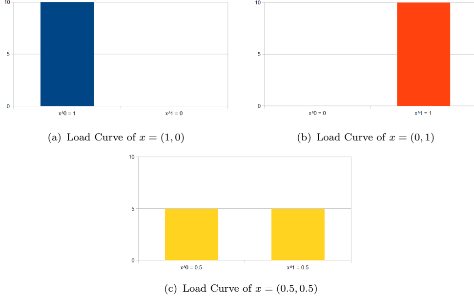
Figure 2: Toy Example
