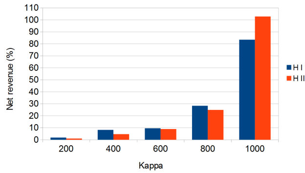
Figure 10: NMP model: Net Revenue Comparison of HI and HII to CEM_{150}(\%) for 200 jobs
