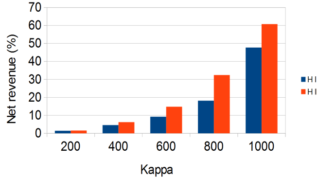
Figure 6: PMP model: Net Revenue Comparison of HI and HII to BC(%) for 100 jobs
