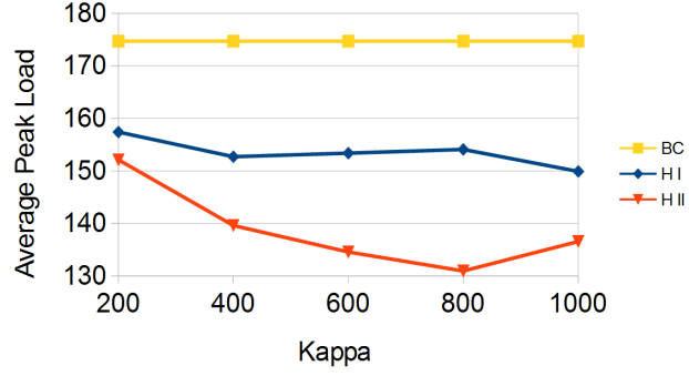
Figure 7: PMP model: Peak Load Comparison of HI and HII to BC for 100 jobs
