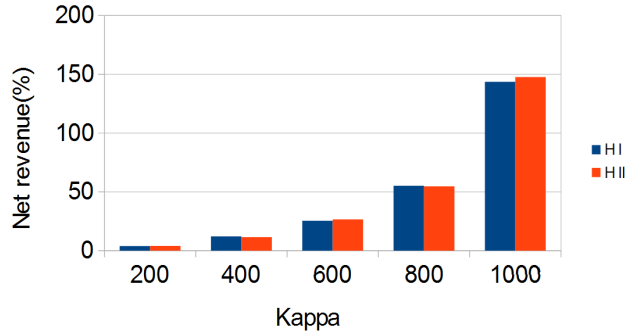
Figure 8: MMP model: Net Revenue Comparison of HI and HII to BC(%) for 100 jobs
