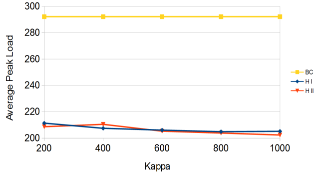
Figure 9: MMP model: Peak Load Comparison of HI and HII to BC for 100 jobs
