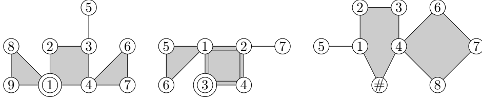
Figure 2: (Left) A hypertree on nine vertices, rooted at 1. (Middle) A hypertree on seven vertices, pointed at edge \{1, 2, 3, 4\} and rooted at 3. (Right) A hollow hypertree on eight vertices. The hollow edge is the edge \{1, 2, 3, 4\} .
