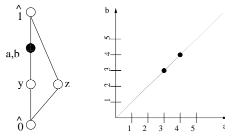
Fig. 9: P_3 and Q_3 are obtained from P and Q by identifying a and b .
