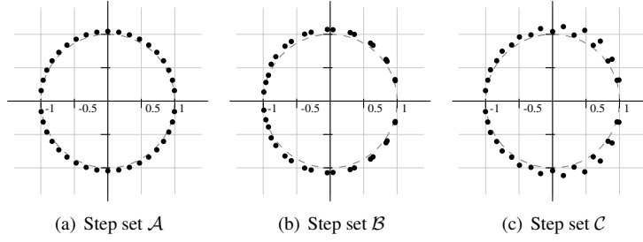
Fig. 1: Plots of the singularities of Y_{20}(1)|_{t=\frac{q}{1+q^2}} for the three symmetric models.
