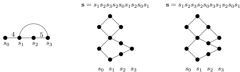
Fig. 1: Two words and their respective heaps.
