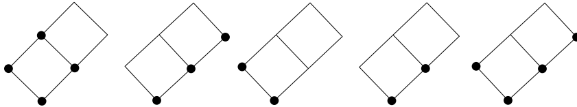
Fig. 1: An orbit of order ideals under the Fon-Der-Flaass action
