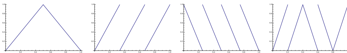
Fig. 1: The graphs of M_\sigma for \sigma = +- , \sigma = +++ , \sigma = --- and \sigma = +-+- , respectively.
