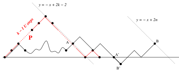
Fig. 6: A forbidden subpath from A to B .
