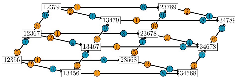
Fig. 2: The positive and negative edge labelings p and n of \mathcal{G}(\mathbb{Q}^{\text{ex}}, \rho^{\text{ex}}) . Each edge has its positive label on the left (orange) and its negative label on the right (blue).
