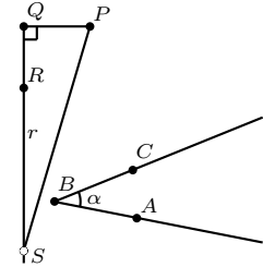
FIGURE 3 – Le postulat de Greenberg.
