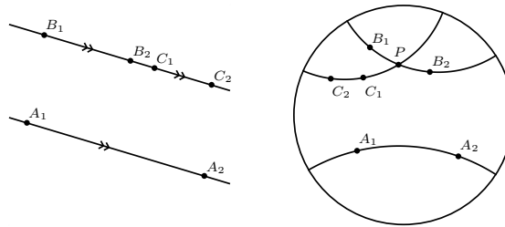
FIGURE 4 – Le postulat de Playfair.
