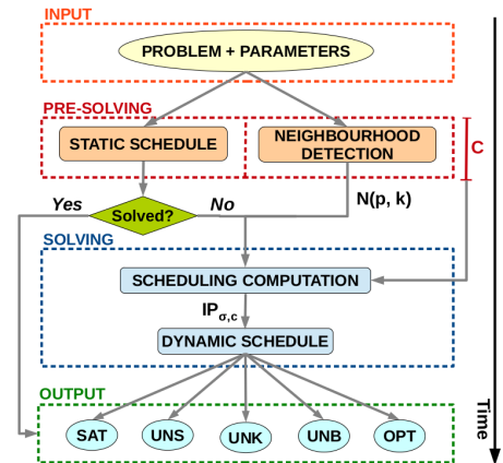
Figure 1: sunny-cp2 architecture.
