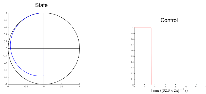
Fig. 3.12 Time-minimal saturation of a single spin ( \lambda = 0.9941 \approx \bar{\lambda} ).
