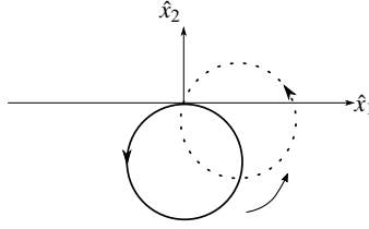
Fig. 2.25 One parameter family of circles which are the geodesics of the Heisenberg-Brockert problem.
