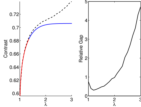
Fig. 3.9 Fluid case. Best upper bounds (dashed line) by the lmi method compared with best solutions by HamPath (solid line), and relative gap between the two.
