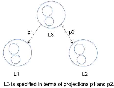
Fig. 5. Language Composition
