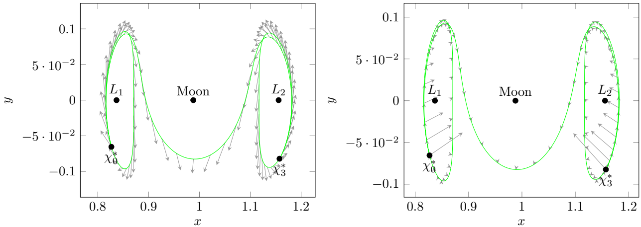
FIGURE 14. Optimal trajectory. On the left the optimal trajectory with \chi_0^* and \chi_3^* fixed on L_{y_1} and L_{y_2} . On the right, the optimal trajectory with \chi_0^* and \chi_3^* free on L_{y_1} and L_{y_2} .
