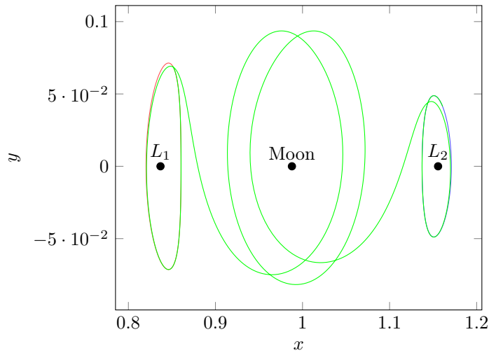
FIGURE 15. Heteroclinic orbit between two Lyapunov orbits in the Earth-Moon system. We get a travel time of 11.699681461946 (normalized time) or 50.883 days.
