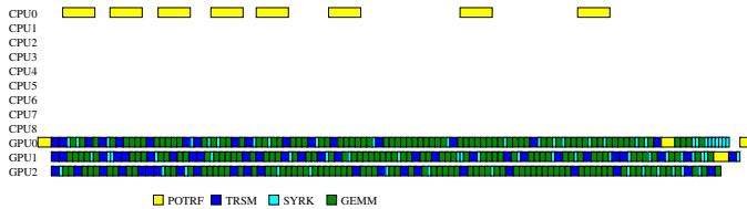
Figure 7. heftp trace for 12 \times 12
