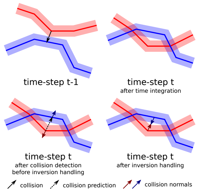
Figure 10: Example of a collision prediction that needs to be re-classified. At time-step t - 1 , two pieces of cloth are in contact; after time integration they enter a colliding state. After collision detection some vertices are not detected as colliding but rather in near collision, because they are at a distance higher than e + e' . Inversion detection is able to correct the normals of the contact point, and the contact point is reclassified as a collision to not be ignored by the physics response.
