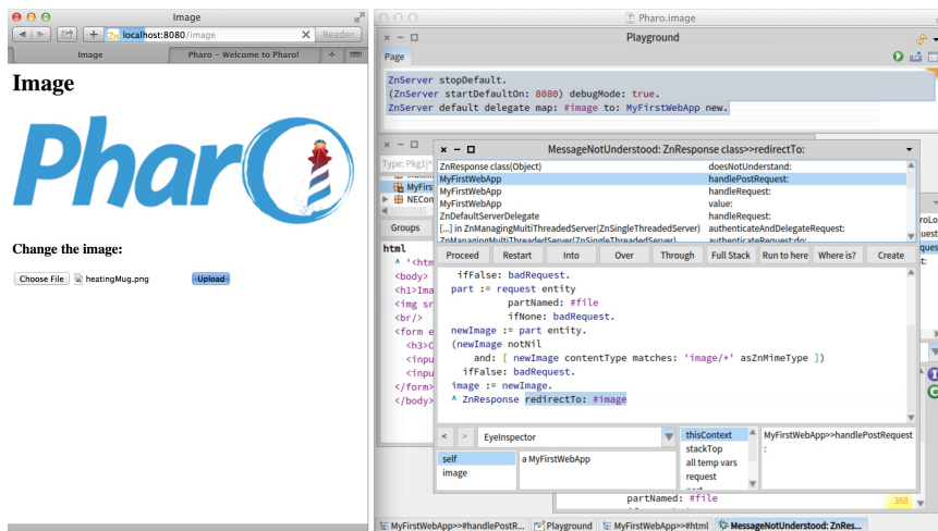
Figure 2.8: Debugging.
