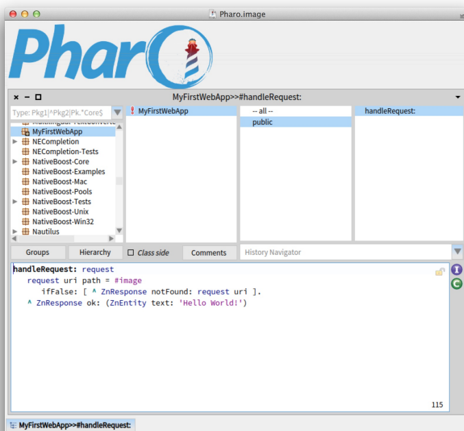
Figure 2.2: Defining a first version of the application.
