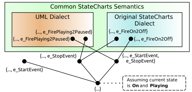
Fig. 6. Simplified event structure showing the Semantic Variation Point of conflicting Transitions .
