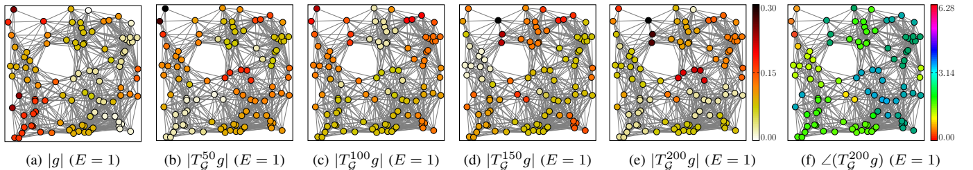
Fig. 1. Random graph as [15, Example 1] with N = 100 , \sigma_1^2 = 1/150 and \sigma_2 = 0.3 . The graph translation operator is iterated on a normalised heat kernel of (a), i.e. on the signal g such that \widehat{g}(\lambda_l) = C e^{-50\lambda_l} . The translated signals being possibly complex, the colour scale illustrates its modulus on (a)-(e) and its phase on (f). See http://perso.ens-lyon.fr/benjamin.girault/ for more figures and animations.
