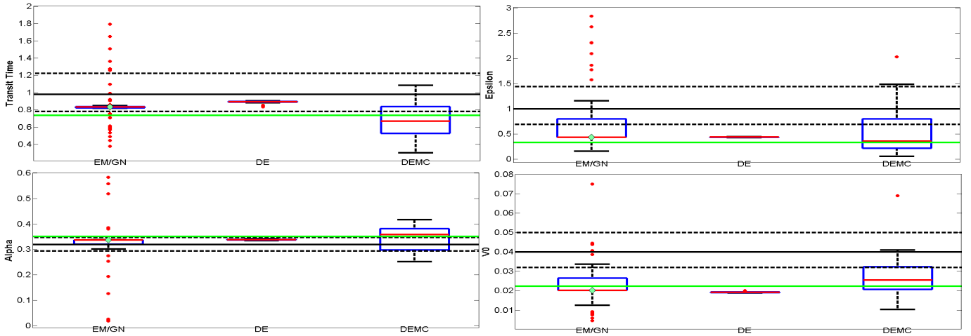
Fig. 1. Boxplots for parameters \alpha, tt, \epsilon, V_0 for synthetic dataset 2. The green horizontal line represents the GT and the diamond displays the estimate achieved using EM/GN from the prior means. Since the actual EM/GN spread is much larger in all cases, we have zoomed-in on a sub-interval to better visualize the differences between the methods. The prior means and prior covariances are displayed as horizontal solid and dashed black lines, respectively.
