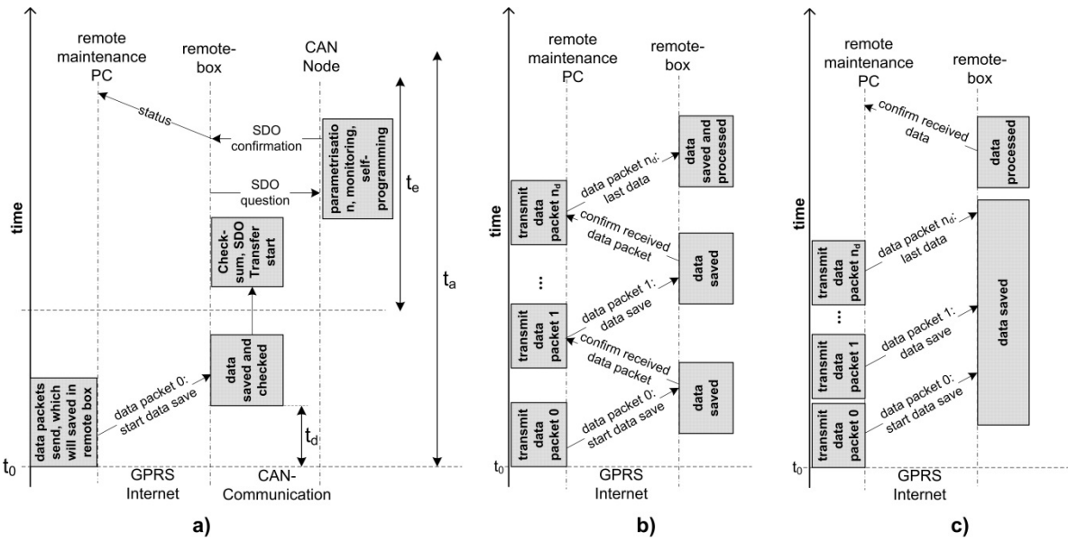
Figure 5: standard transmit processes
