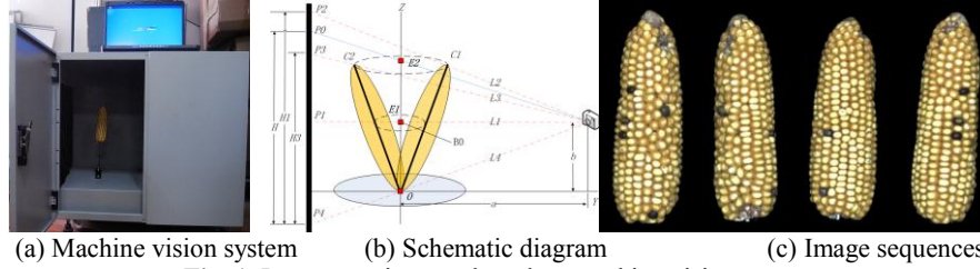
Fig. 1. Image acquirement based on machine vision system
