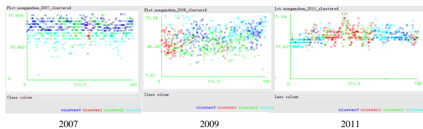
Fig. 3. Clustering results
