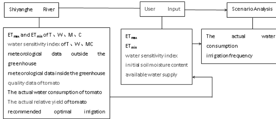
Fig.2.data structure
