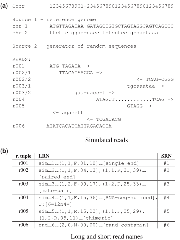
Fig. 1. Examples of simulated reads (in our definition read tuples) and their corresponding RNF names, which can be used as read names in the final FASTQ file: a single-end read (r001); a paired-end read (r002); a mate-pair read (r003); a spliced RNA-seq read (r004); a chimeric read (r005); and a random contaminating read with unspecified coordinates (r006)
