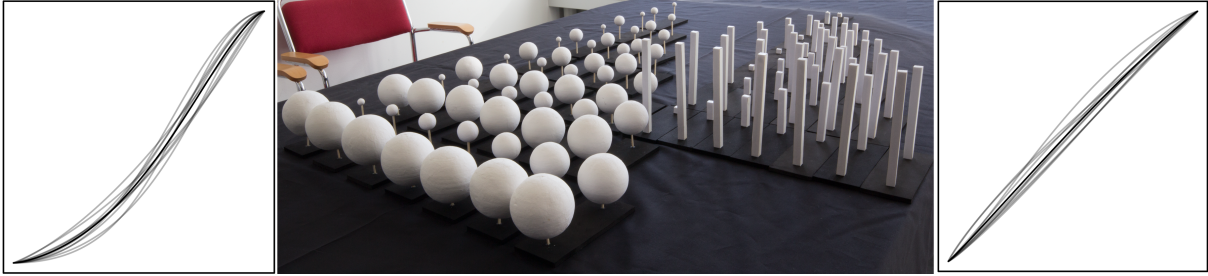
Fig. 1. Middle: the pairs of physical marks used during the experiment. Left and right: fitted psychophysical response curves for spheres and bars respectively, overplotted to show individual curves for all participants.
