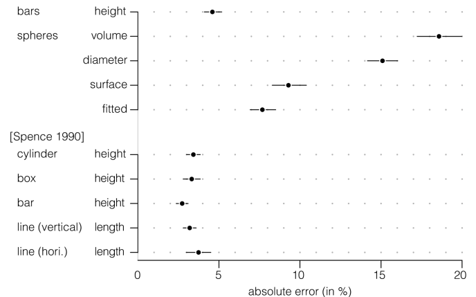
Fig. 11. Dot plot of absolute errors for bars and spheres computed for different objective measures. Error bars indicate 95% bootstrapped confidence intervals. Data for Spence taken from [50].
