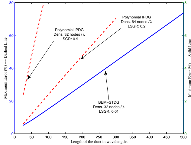
Figure 11: Maximum error in % for polynomial approximations of degree m = 1 . The left y -axis corresponds to the error curves of the IPDG method and the right y -axis to the BEM-STDG method.
