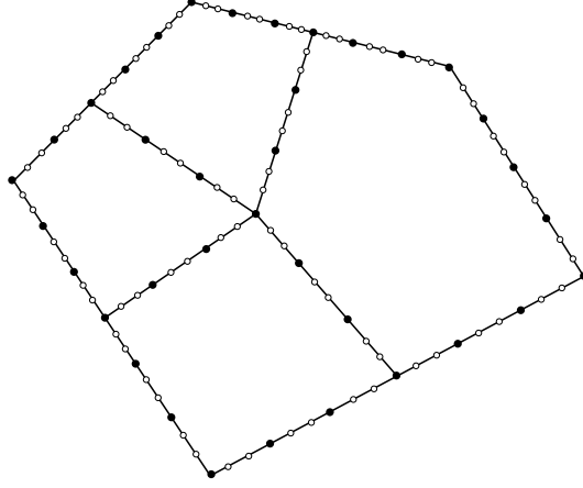
Figure 4: Schematic view of the three kinds of meshes, which are used in the BEM-STDG method. The 4 polygonals constitute the interior mesh. The vertices of the skeleton and the refined meshes are marked by large dots and small circles respectively. The refinement parameter N_{\text{add}} is taken equal to 3 here.
