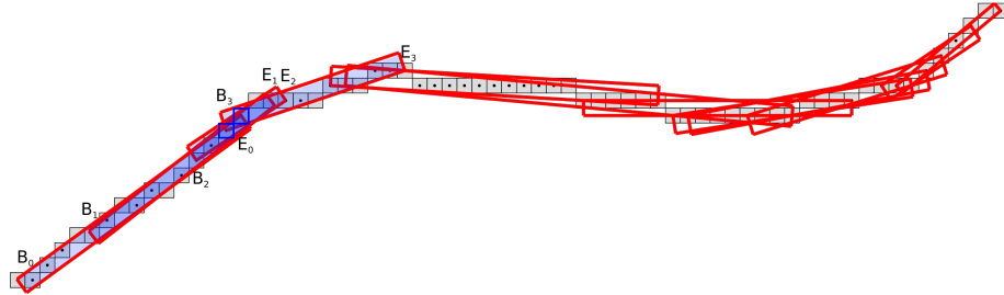
Fig. 2. A sequence of width 1.4 maximal blurred segments of the curve with grey pixels (each red box bounds the pixels of a maximal blurred segment of width 1.4). The indexes of the begin ( B_i ) and end ( E_i ) points of the four first maximal blurred segments are indicated ( B_0 = 0 and E_0 = 15 , B_1 = 5 and E_1 = 17 , ...). The points with blue frame are points in the common zone – intersecting zone – defined by these four first maximal blurred segments.
