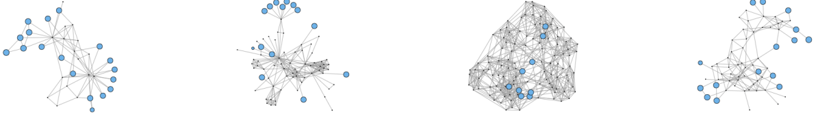
Fig. 1: Visualization of the solution of the Katz-Bonacich centrality minimization problem
