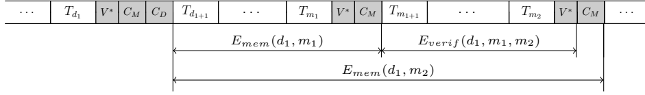
Figure 2: Placing memory checkpoints.
