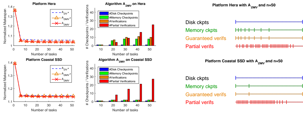
Figure 7: Performance of the three algorithms, and distribution of disk checkpoints, memory checkpoints and verifications (for the A_{DMV} algorithm) on platforms Hera and Coastal SSD with the Decrease pattern.
