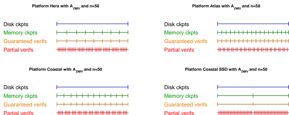
Figure 6: Distribution of disk checkpoints, memory checkpoints and verifications for the A_{DMV} algorithm on each platform with the Uniform pattern.
