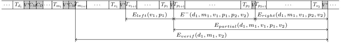
Figure 4: Placing partial verifications.
