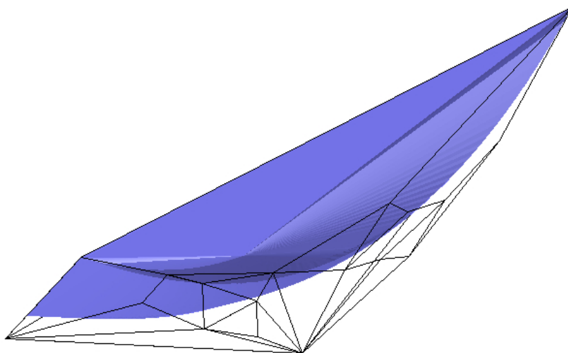
Fig. 8: The convex hull of the curvy zonotope Z_{(K_3, C_4, K_4 \setminus e); 2} in Figure 7.
