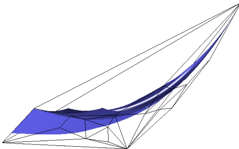
Fig. 7: The curvy zonotope Z_{(K_3, C_4, K_4 \setminus e); 2} inscribed in P_{(K_3, C_4, K_4 \setminus e); 6} from Figure 1.
