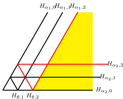
Fig. 3: There are three regions in \mathfrak{h}_{\alpha_1 2}^3
