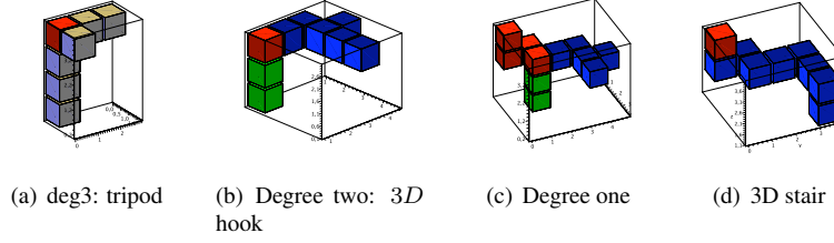
Fig. 2: Corner polyominoes
