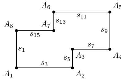
Fig. 8: An axis-aligned octagon. The side lengths s_3, s_5, s_7, and s_9 are positive and the others are negative.
