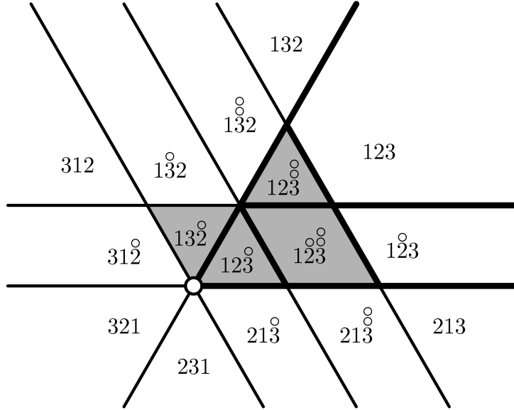
Fig. 7: The arrangement \text{Ish}(3) labeled with Ish ceiling diagrams
