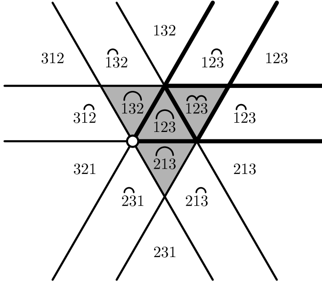
Fig. 5: The regions of Shi(3) and their Shi ceiling diagrams.
