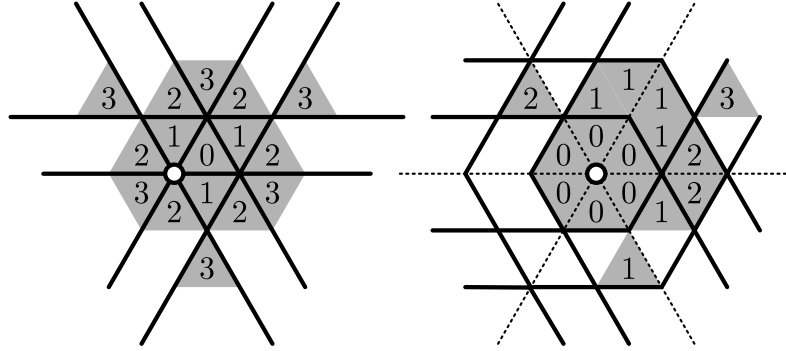
Fig. 4: The shi and ish statistics on the chambers of \text{Shi}(3)
